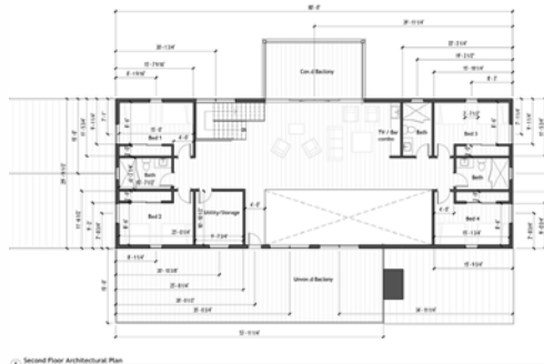
⑤ Second Floor Architectural Plan 1/8" = 1'-0"
